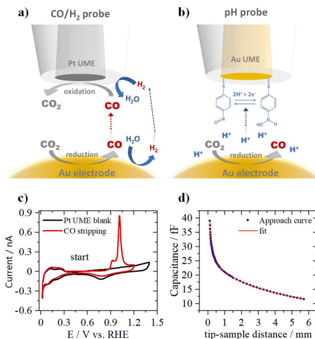
Figure 1. Schematic representation of (a) the SG-TC collection mode of SECM, where a Pt-UME is used to probe CO and H 2 while CO 2 reduction takes place at the gold sample, (b) the functionalized Au-UME used to measure pH, and (c) Pt-UME blank voltammetry (black) taken in argon-saturated 0.1 M \text{H}_2\text{SO}_4 and CO stripping voltammetry measured in the same electrolyte after exposing the Pt-UME to a CO atmosphere for 5 min. CVs taken at 200 mV s −1 . (d) Capacitive approach curve to determine the absolute tip-to-surface distance.
