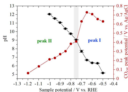
Figure 4. Correlation between the pH measurements performed with a functionalized Au-UME (black circles) with the CO oxidation peak position extracted from the measurements performed with the Pt-UME (red circles) during \text{CO}_2 reduction on gold ( 0.1 \text{ M Cs}_2\text{SO}_4 , \text{pH} = 3 , \text{CO}_2 saturated).
