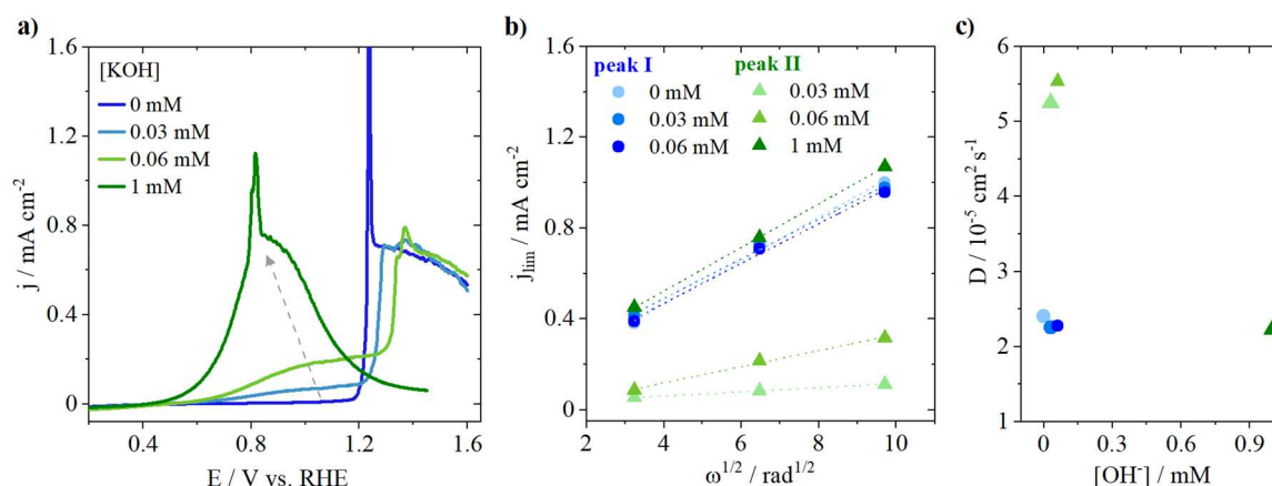
Figure 5. RDE CO oxidation measurements on a polycrystalline Pt disc in \text{Cs}_2\text{SO}_4 (pH = 7.2) performed at 400 rpm with a 25 \text{ mV s}^{-1} scan rate. (a) Reaction performed in the presence of different concentrations of KOH, (b) Levich plot, and (c) derivation of the diffusion coefficients for peak I (blue circles) and peak II (green triangles).
